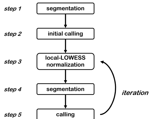
Figure 1: Overview of the CGHnormaliter method.
