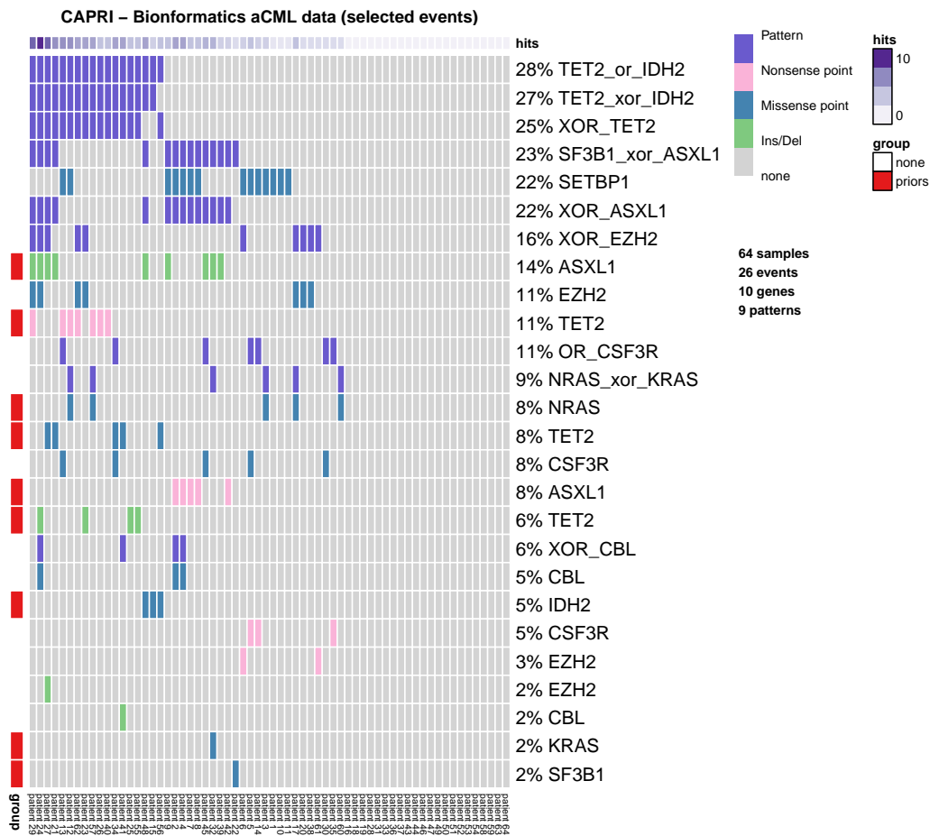
Figure 8: oncoprint output of the dataset that has patterns that could be given as input to CAPRI to retrieve a progression model
