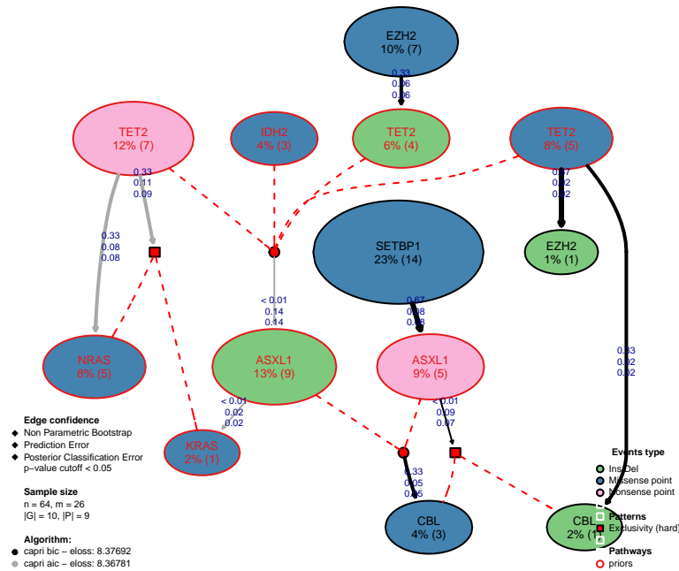
Figure 15: aCML model reconstructed by CAPRI with AIC/BIC as regularizers and annotated with non-parametric, as well as with entropy loss, prediction and posterior classification errors computed via cross-validation Edge thickness is proportional to the non-parametric scores.
