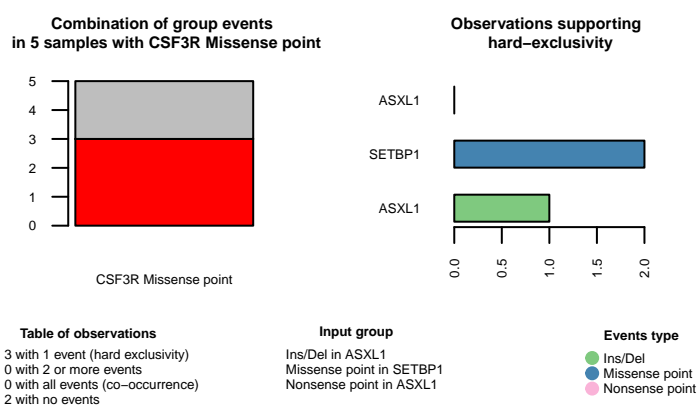
Figure 9: Barplot to show an hypothesis: here we test genes SETBP1 and ASXL1 versus Missense point mutations of CSF3R, which suggests that that pattern does not “capture” all the samples with CSF3R mutations
