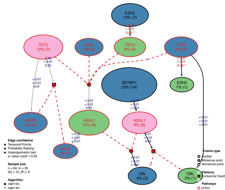
Figure 11: aCML model reconstructed by CAPRI with AIC/BIC as regularizers; the confidence of each edge is shown both in terms of temporal priority and probability raising (selective advantage scores) and hypergeometric testing (statistical relevance of the dataset of input)
