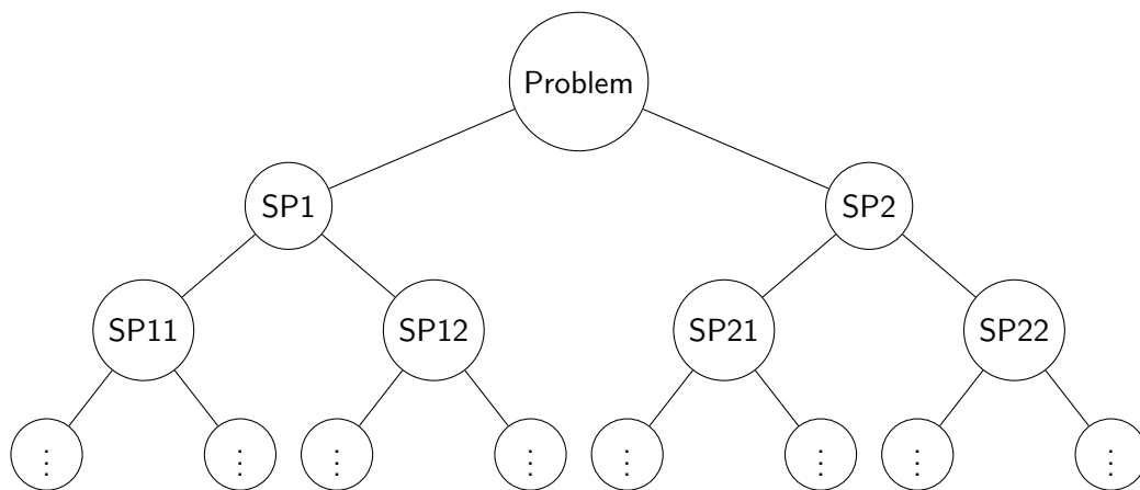
Figure 2: A sketch of a search tree generated by branch and bound
