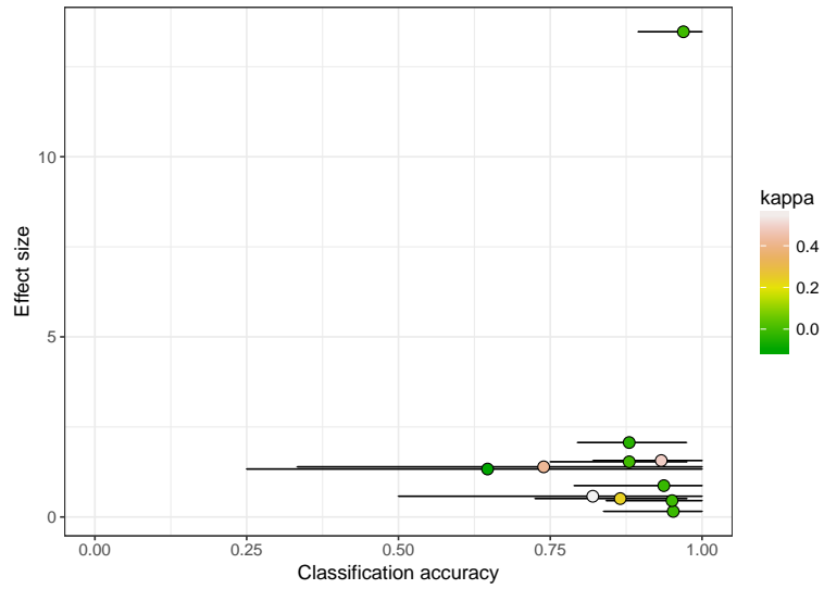
Figure 3: Effect site - classification accuracy plot
